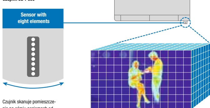
Czujnik 3D i-see
